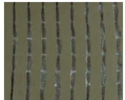
Kleberbild / Normalzahnung. Mortar structure with conventional notched trowel
